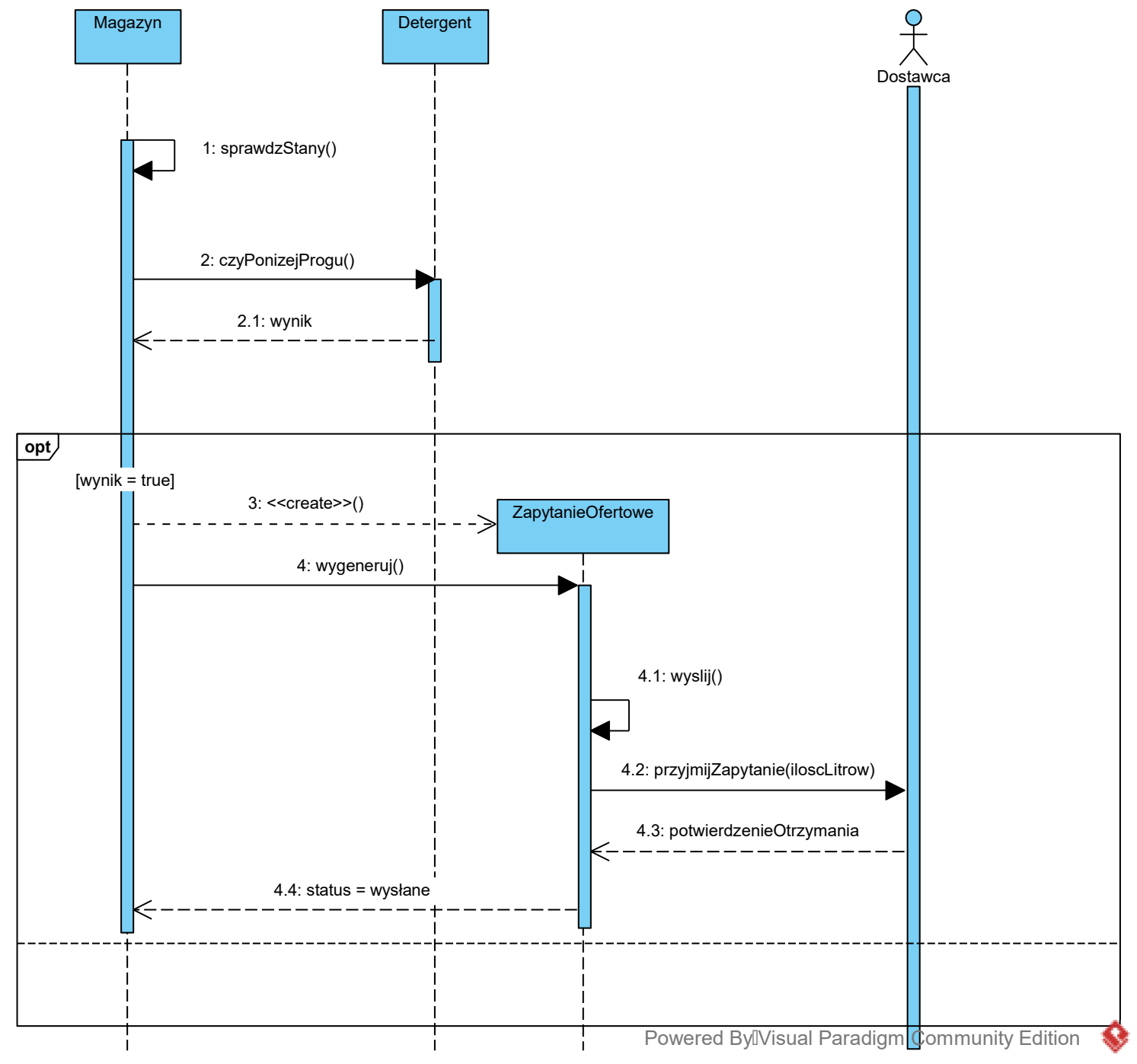
sd [Sequence Diagram3]
